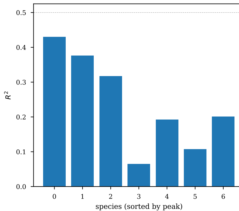
E) Per-species growth-rate R^2
