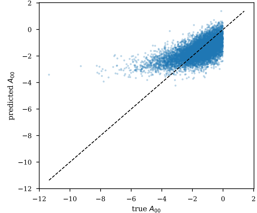
C) Best A entry — R^2=0.393
