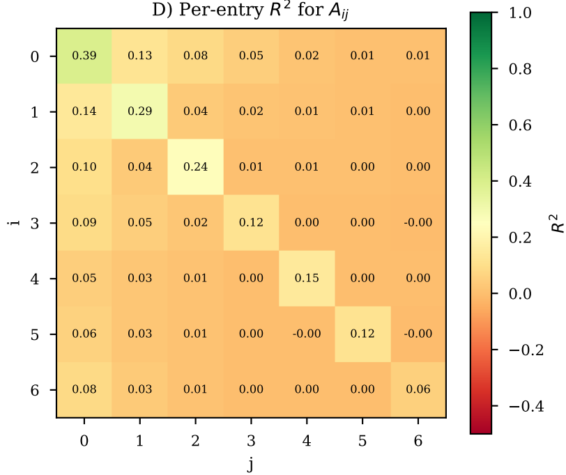
D) Per-entry R^2 for A_{ij}
