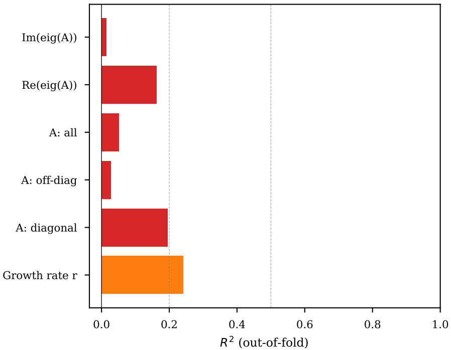
A) Parameter recoverability from \mu(z)
